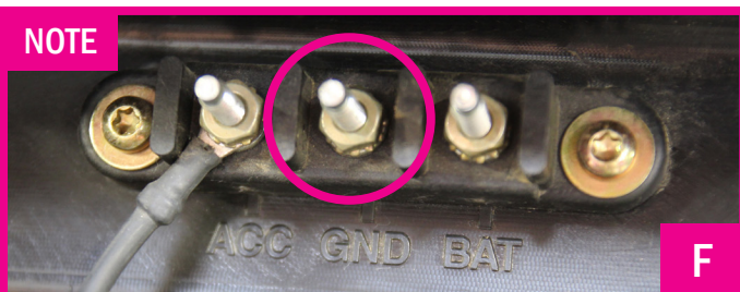
F. Some RZR models come with the ground "GND" terminal not connected as shown. If you do not have a factory wiring going to this terminal, add a ground wire from the "GND" terminal to the frame before connecting the wires. We recommend removing the paint to bare metal, using a star washer, and repainting over the connection.
