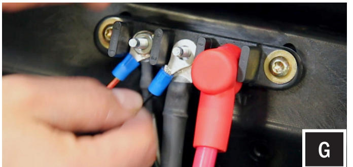
G. Run the (RED) Power and (BLACK) Ground wire of the USB/Aux input port to the Bus Bar. Unscrew the nut on the first position terminal (accessory) and attach the (RED) Power wire. Re-screw on the nut. Then unscrew the nut on the second position terminal and attach the (BLACK) Ground wire. Re-screw on the nut.
