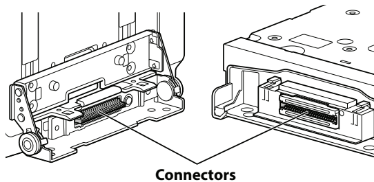
<Display unit>
