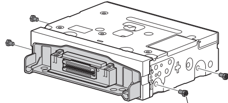
Hexagon bolts ×4
